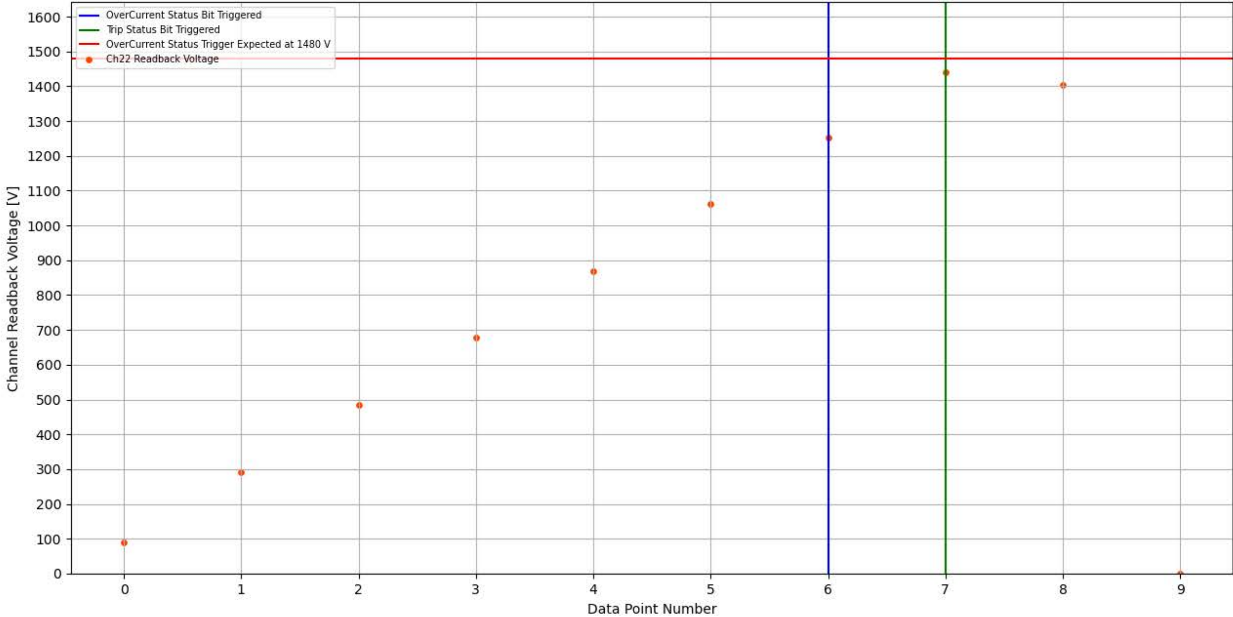
Module 352, Slot 2, Channel 22 Trip Test
