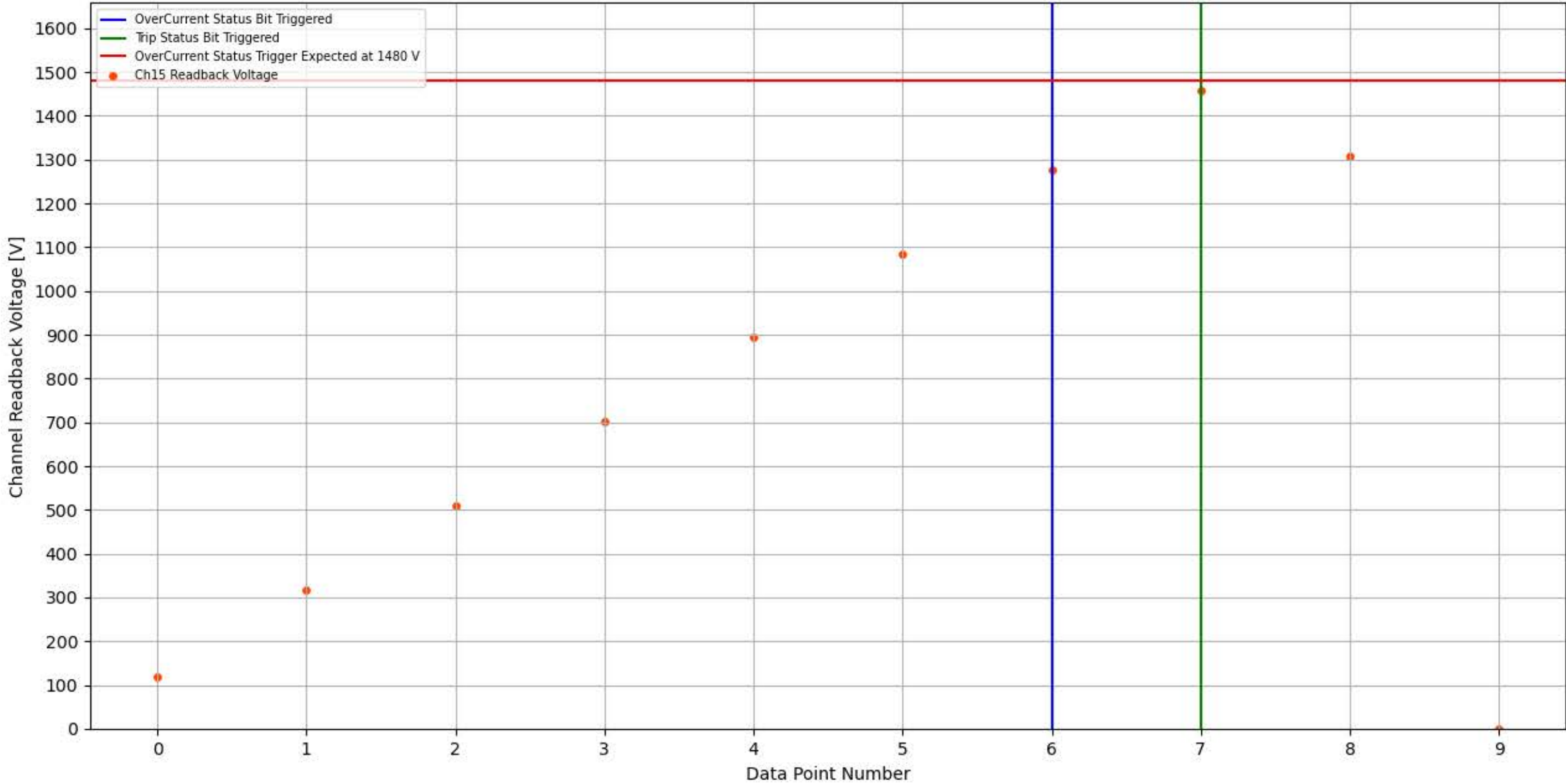
Module 352, Slot 2, Channel 15 Trip Test
