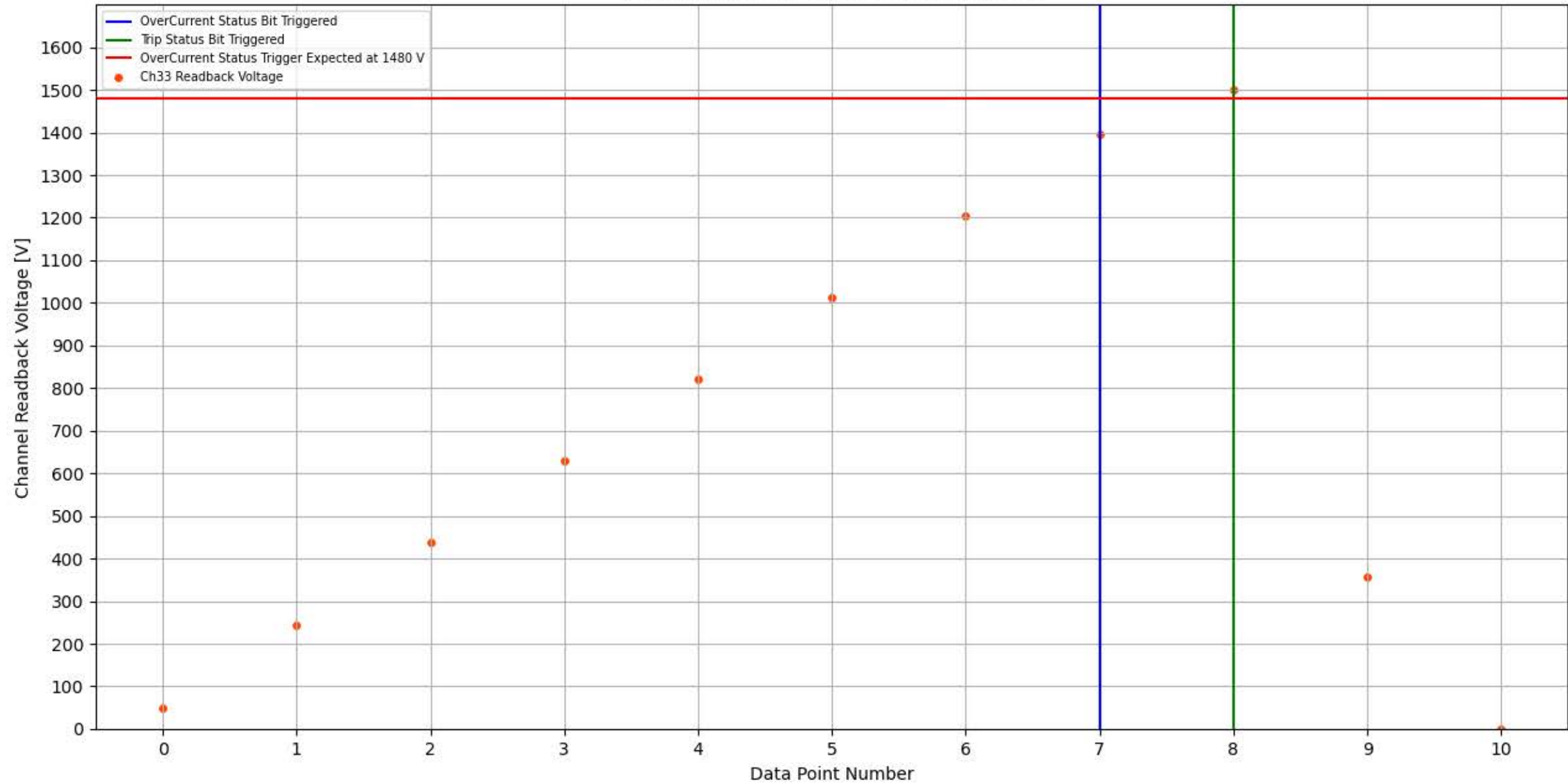
Module 352, Slot 2, Channel 33 Trip Test
