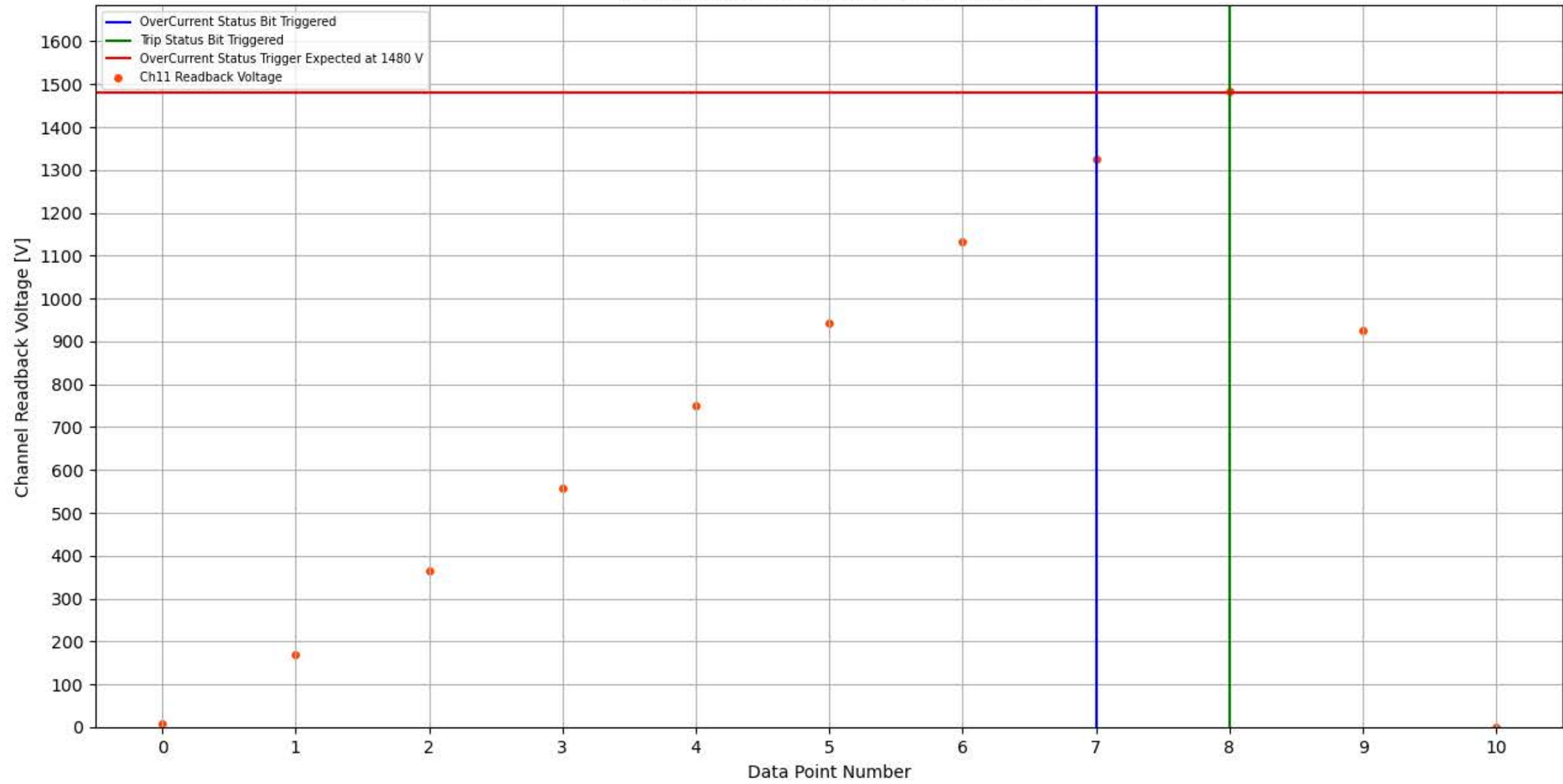
Module 352, Slot 2, Channel 11 Trip Test
