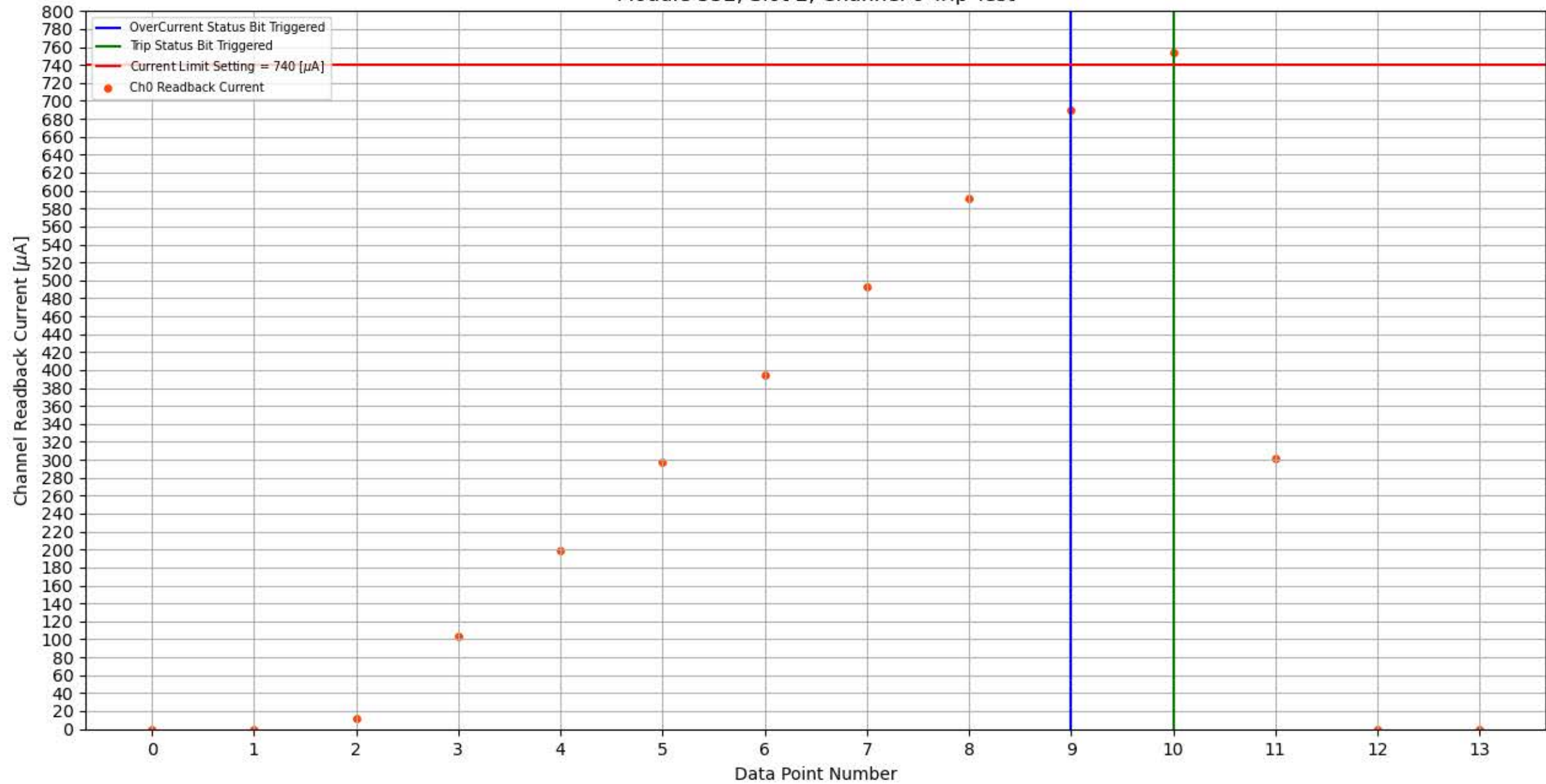
Module 352, Slot 2, Channel 0 Trip Test
