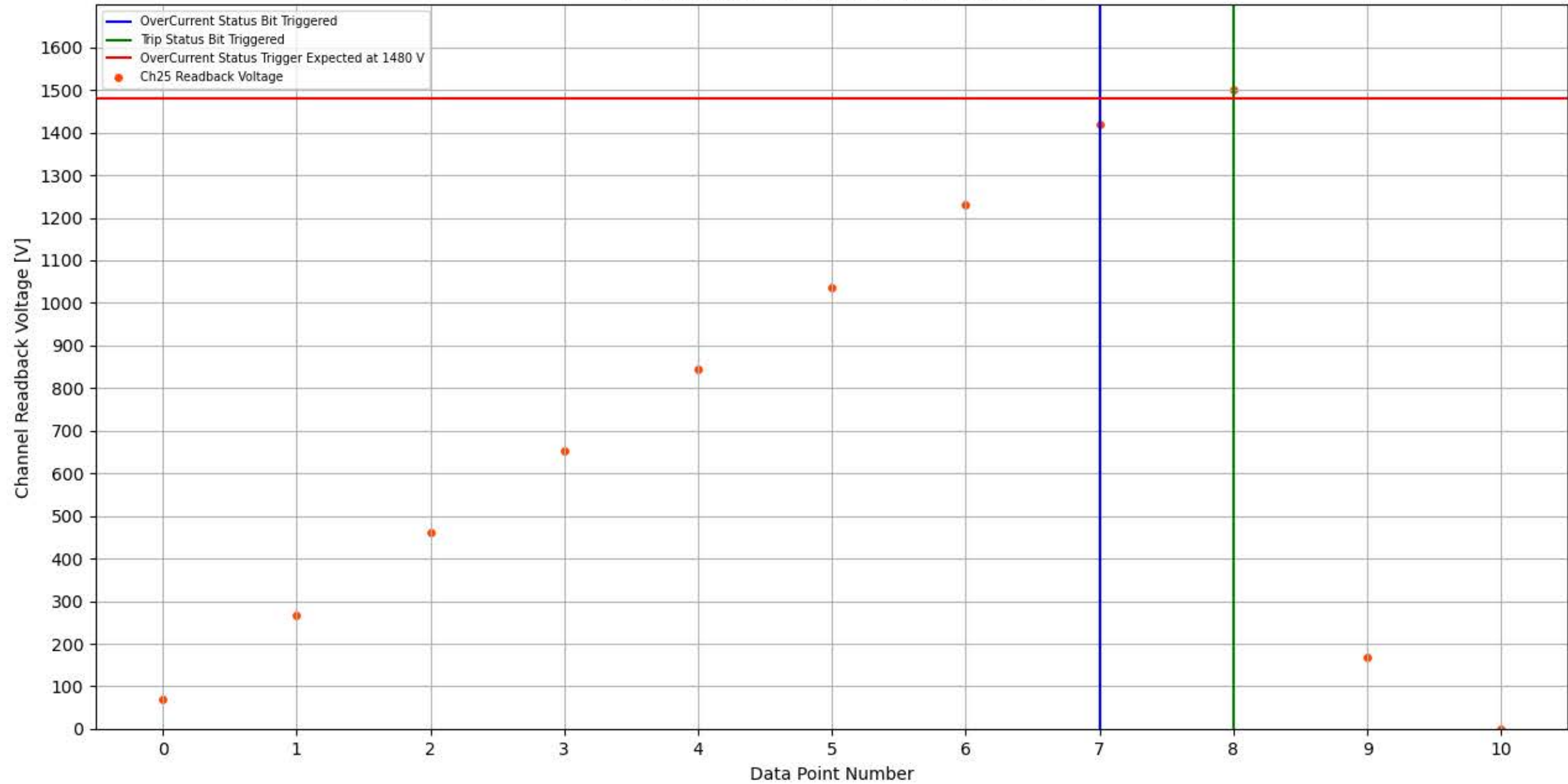
Module 352, Slot 2, Channel 25 Trip Test
