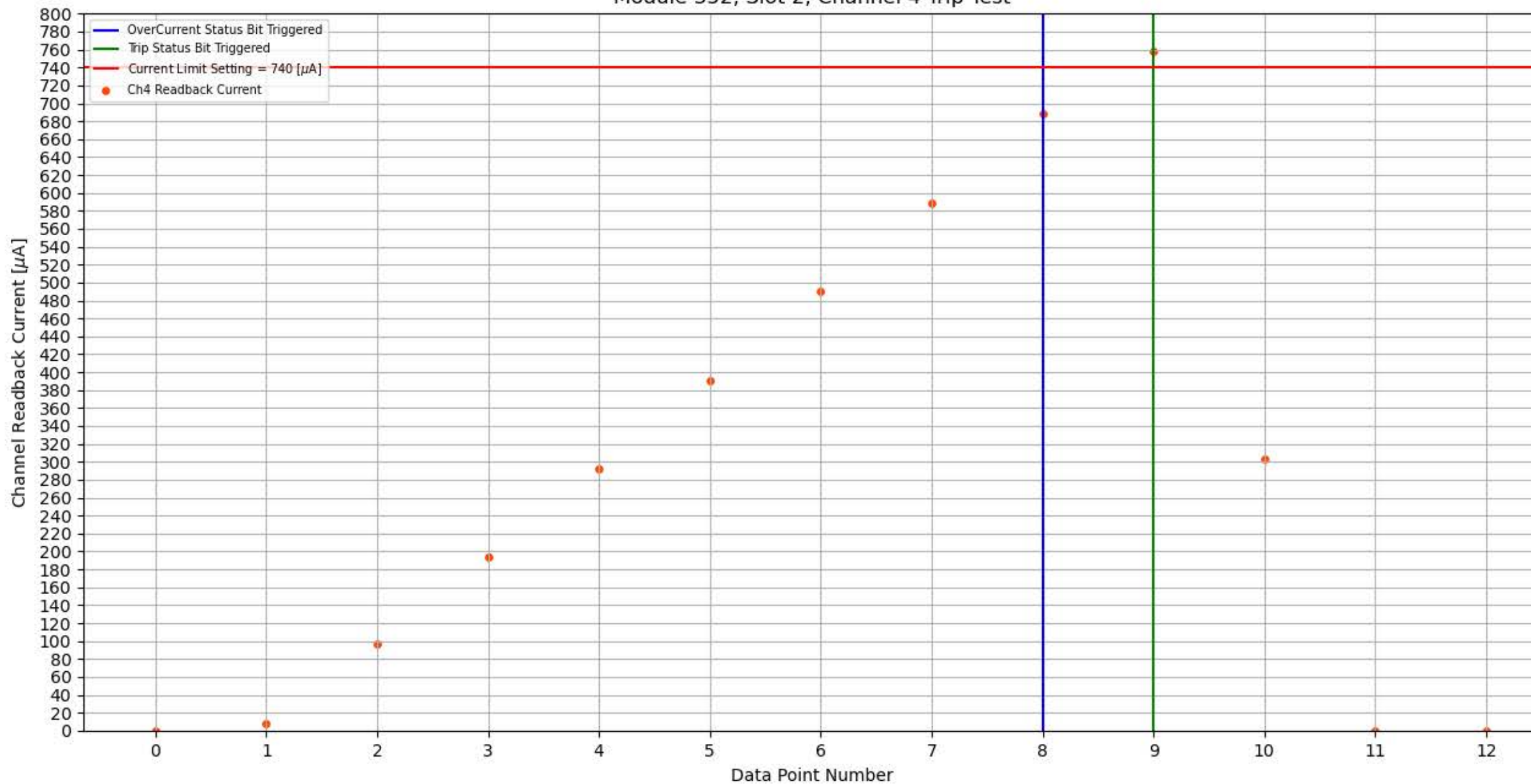
Module 352, Slot 2, Channel 4 Trip Test
