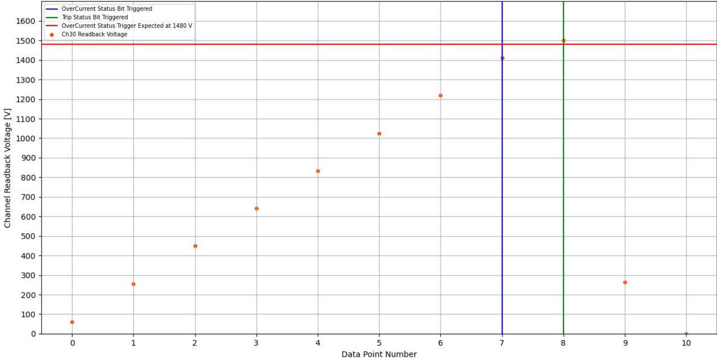
Module 352, Slot 2, Channel 30 Trip Test
