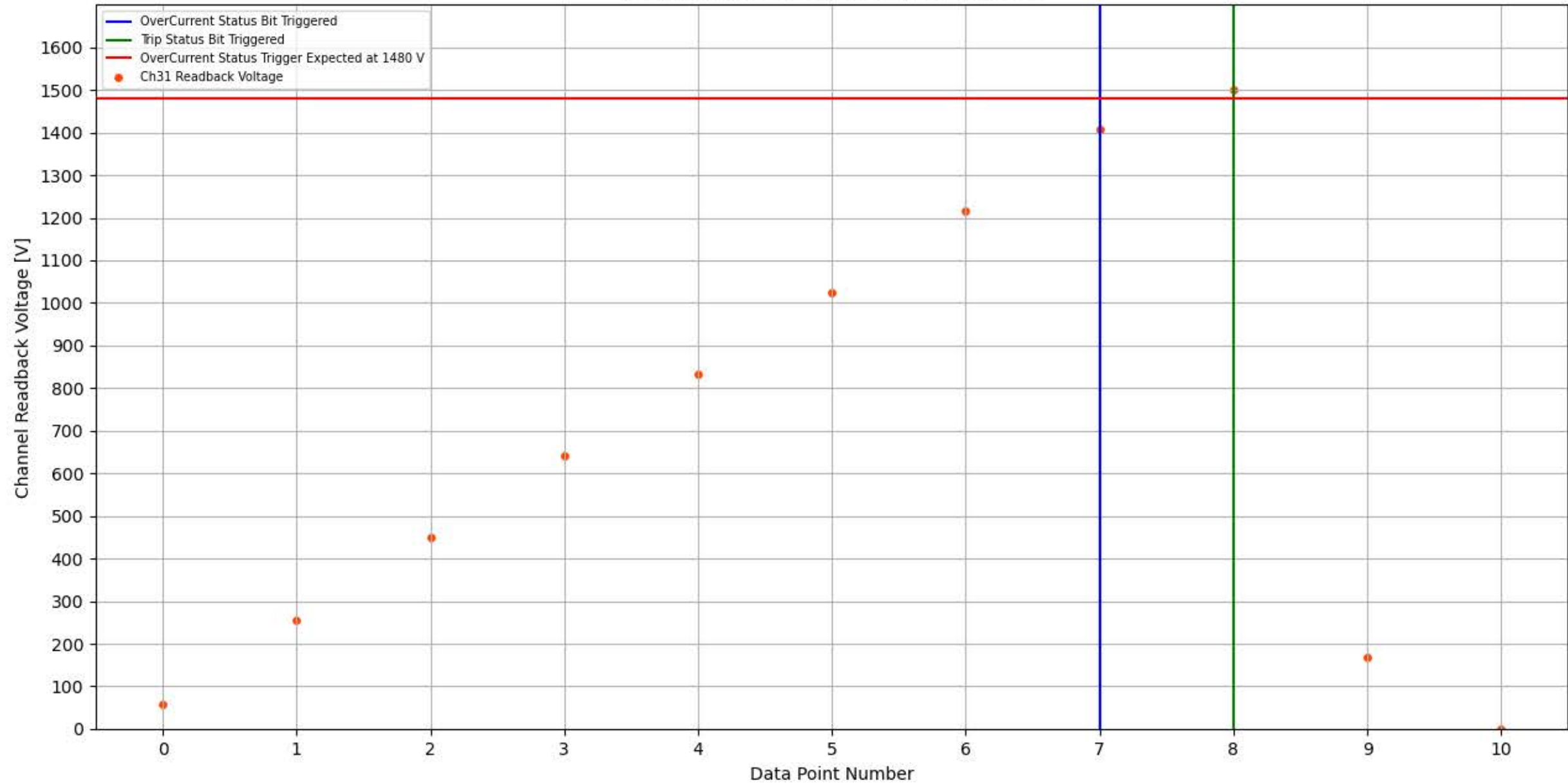
Module 352, Slot 2, Channel 31 Trip Test
