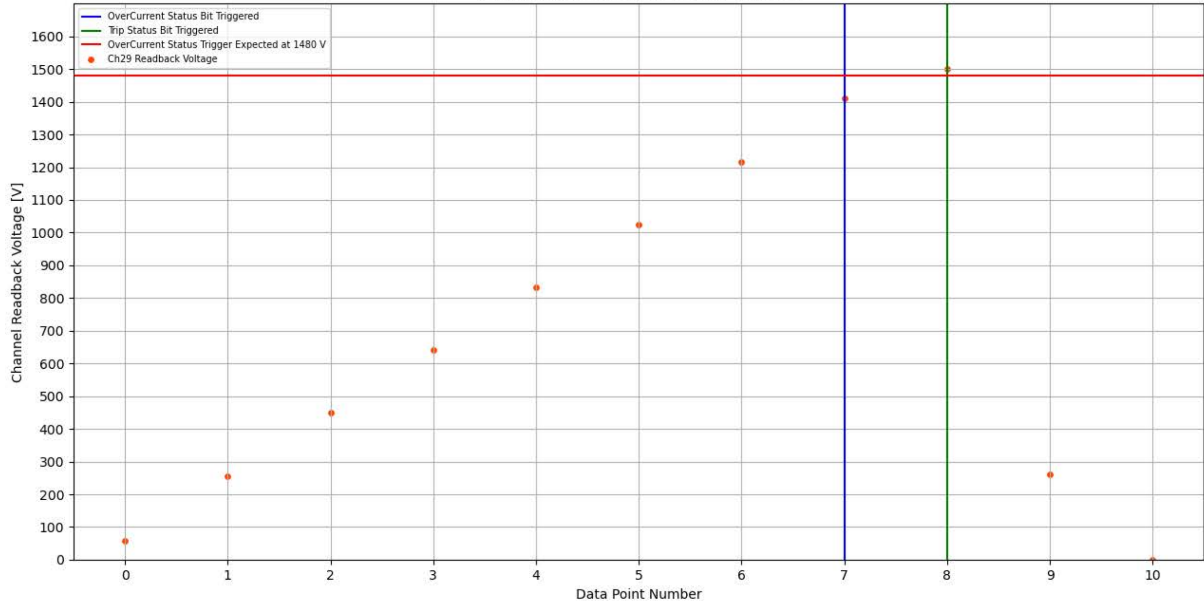
Module 352, Slot 2, Channel 29 Trip Test
