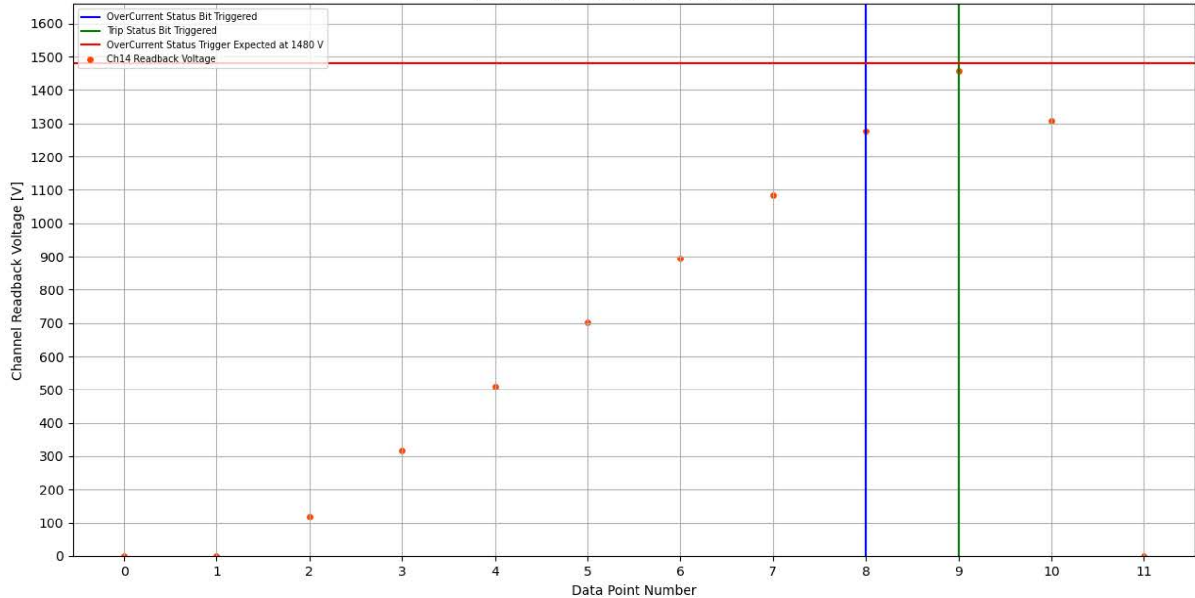
Module 352, Slot 2, Channel 14 Trip Test
