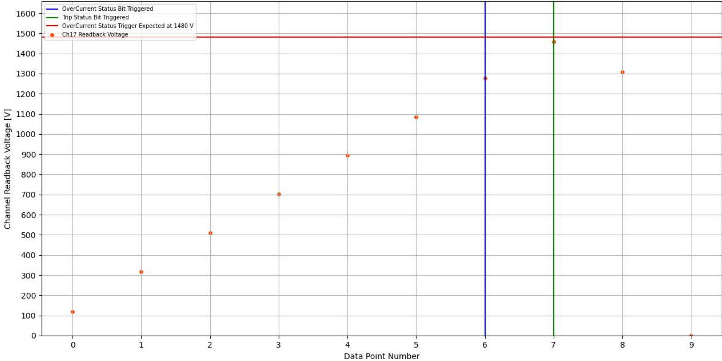
Module 352, Slot 2, Channel 17 Trip Test
