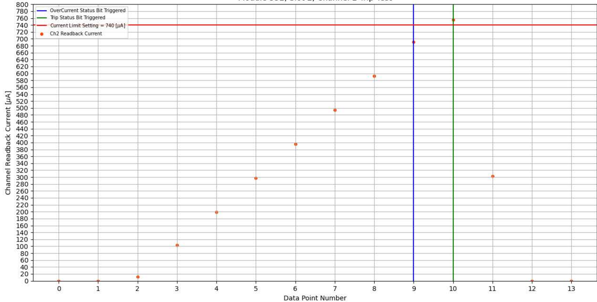
Module 352, Slot 2, Channel 2 Trip Test
