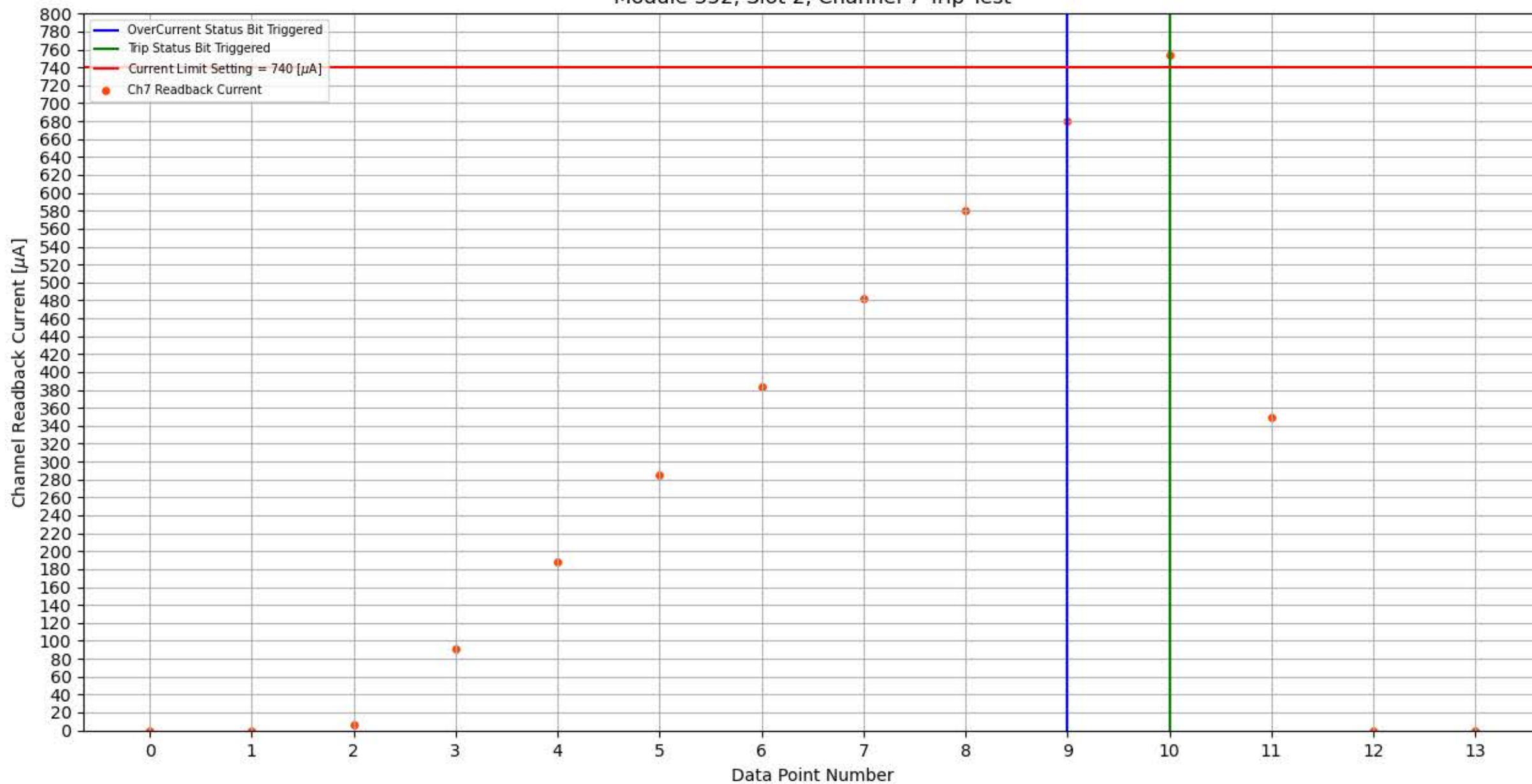
Module 352, Slot 2, Channel 7 Trip Test
