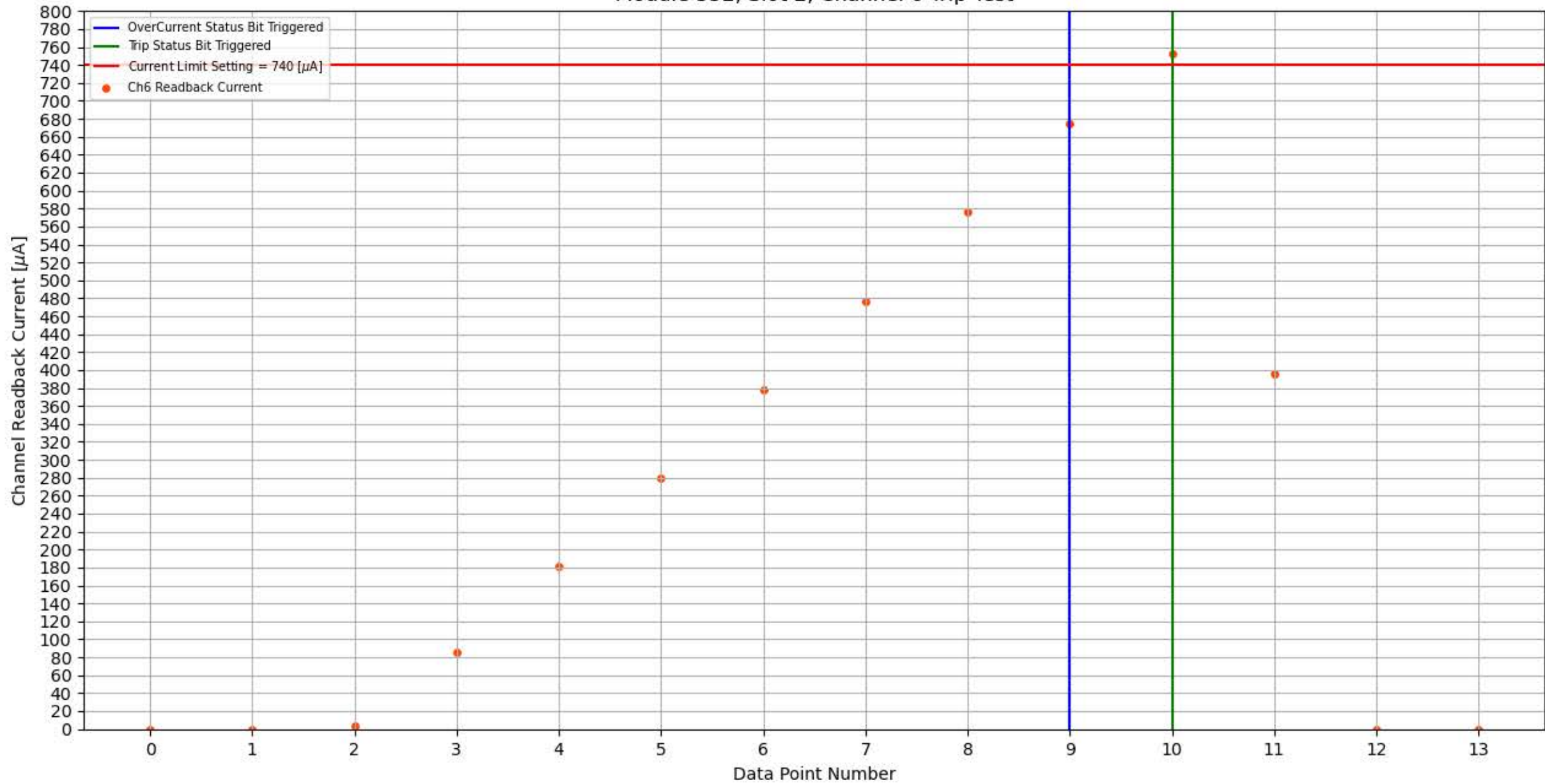
Module 352, Slot 2, Channel 6 Trip Test
