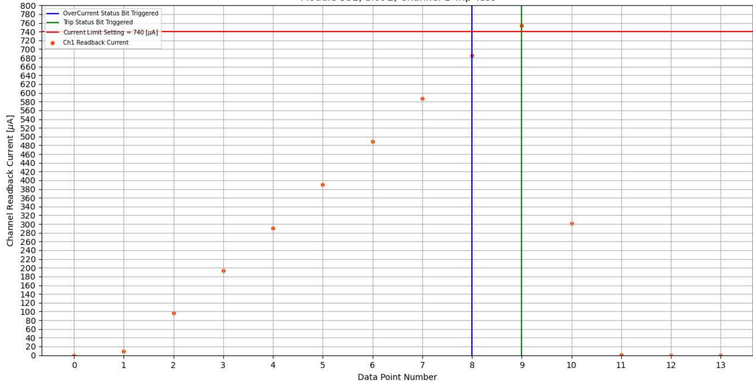
Module 352, Slot 2, Channel 1 Trip Test
