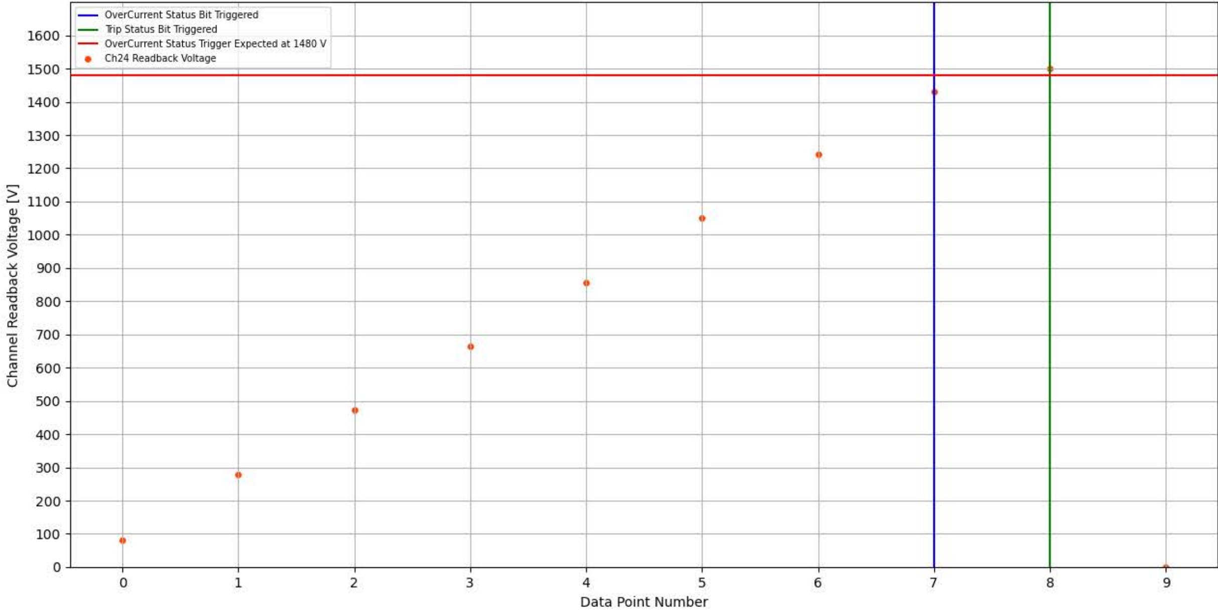
Module 352, Slot 2, Channel 24 Trip Test
