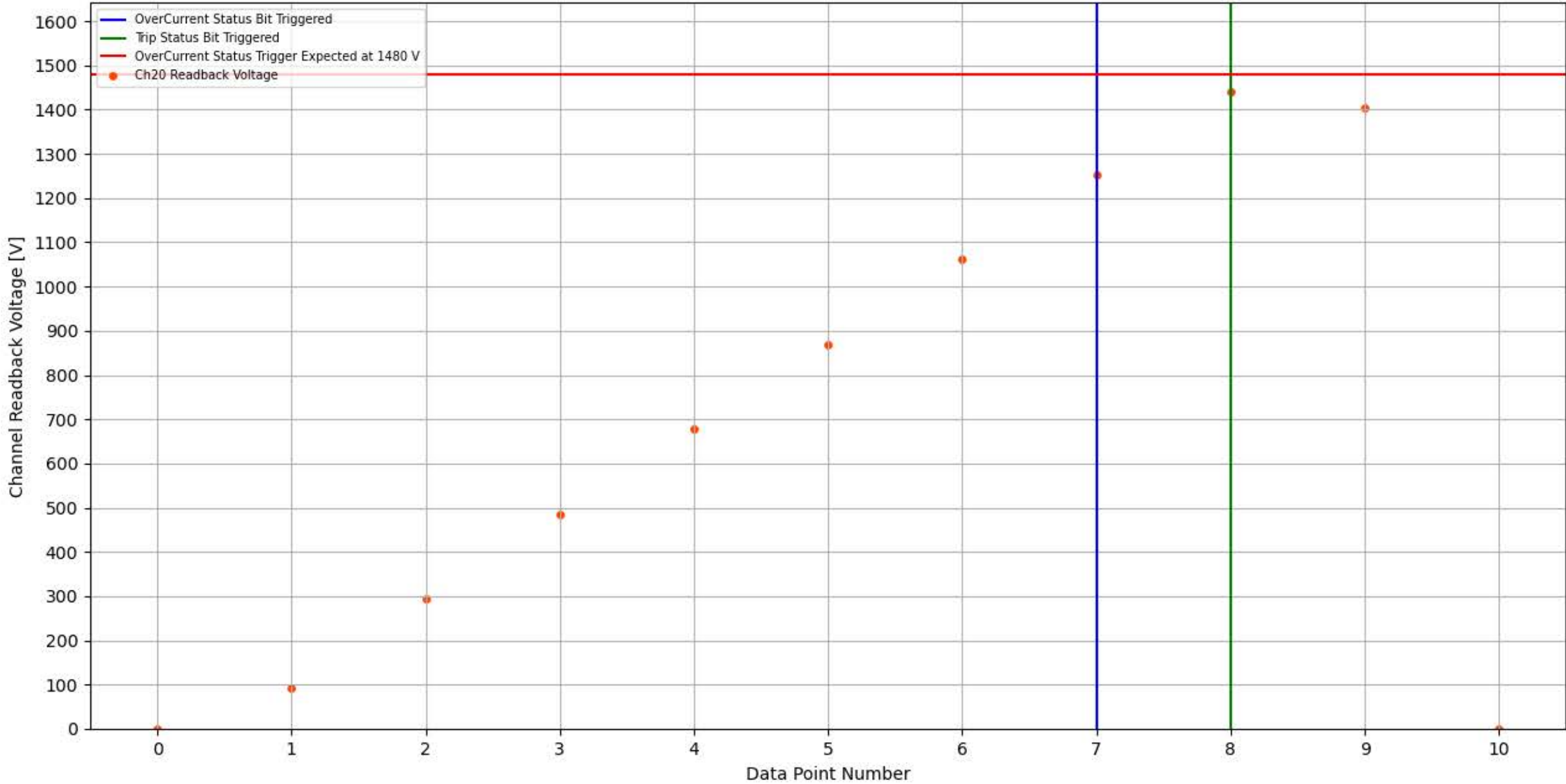
Module 352, Slot 2, Channel 20 Trip Test
