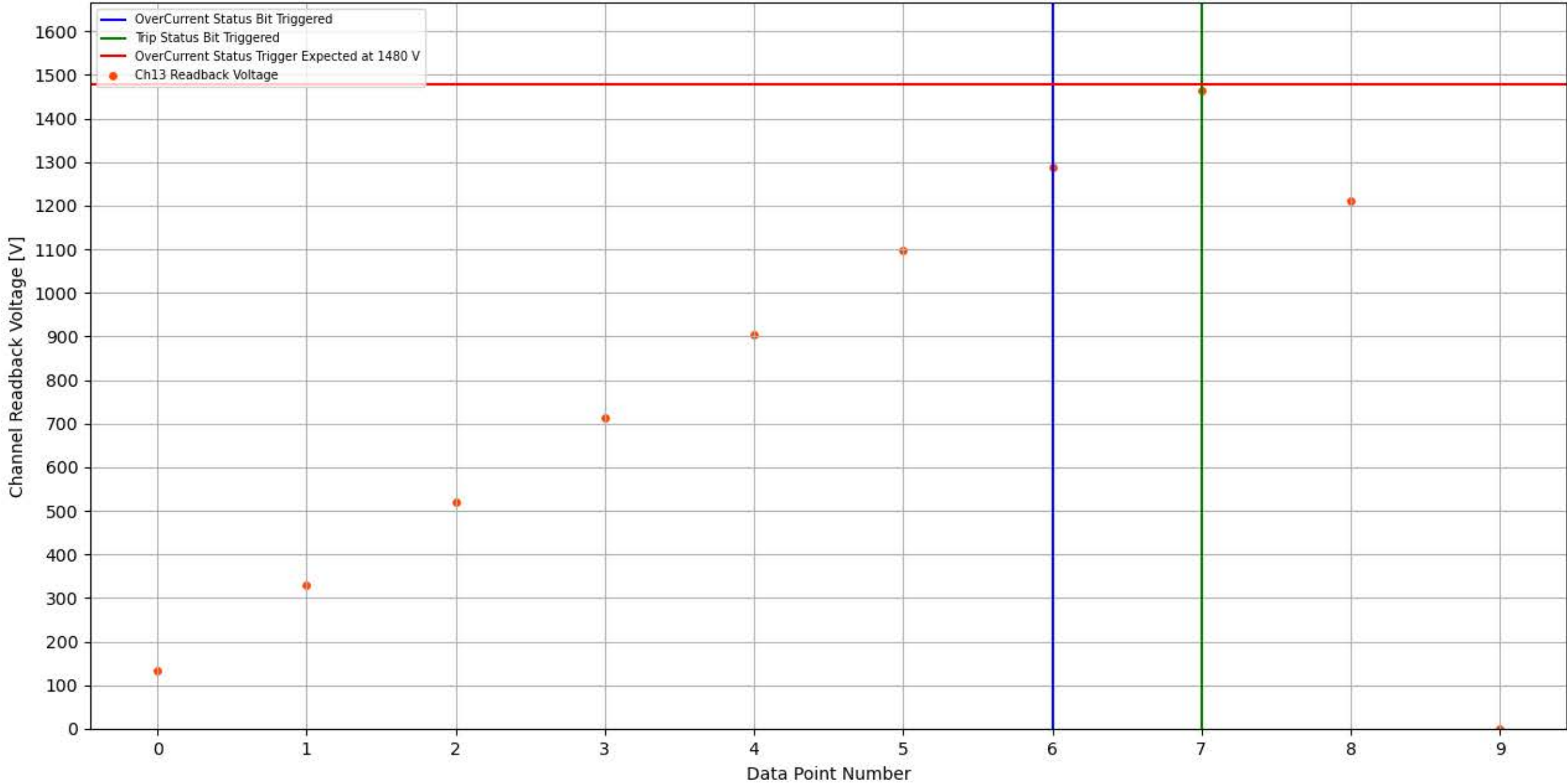
Module 352, Slot 2, Channel 13 Trip Test
