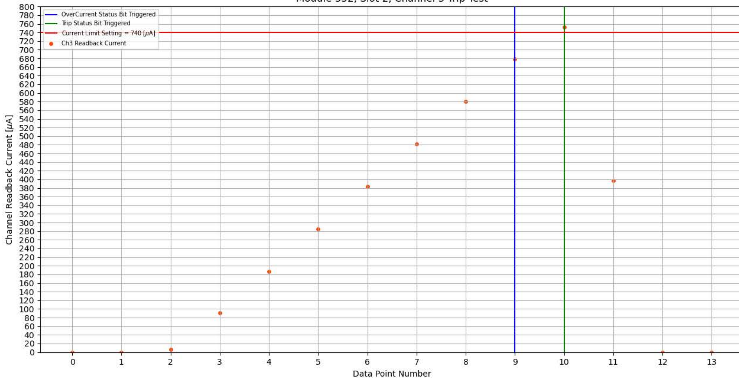
Module 352, Slot 2, Channel 3 Trip Test
