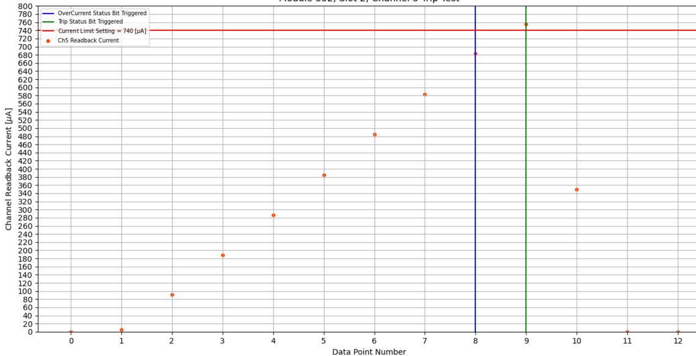
Module 352, Slot 2, Channel 5 Trip Test
