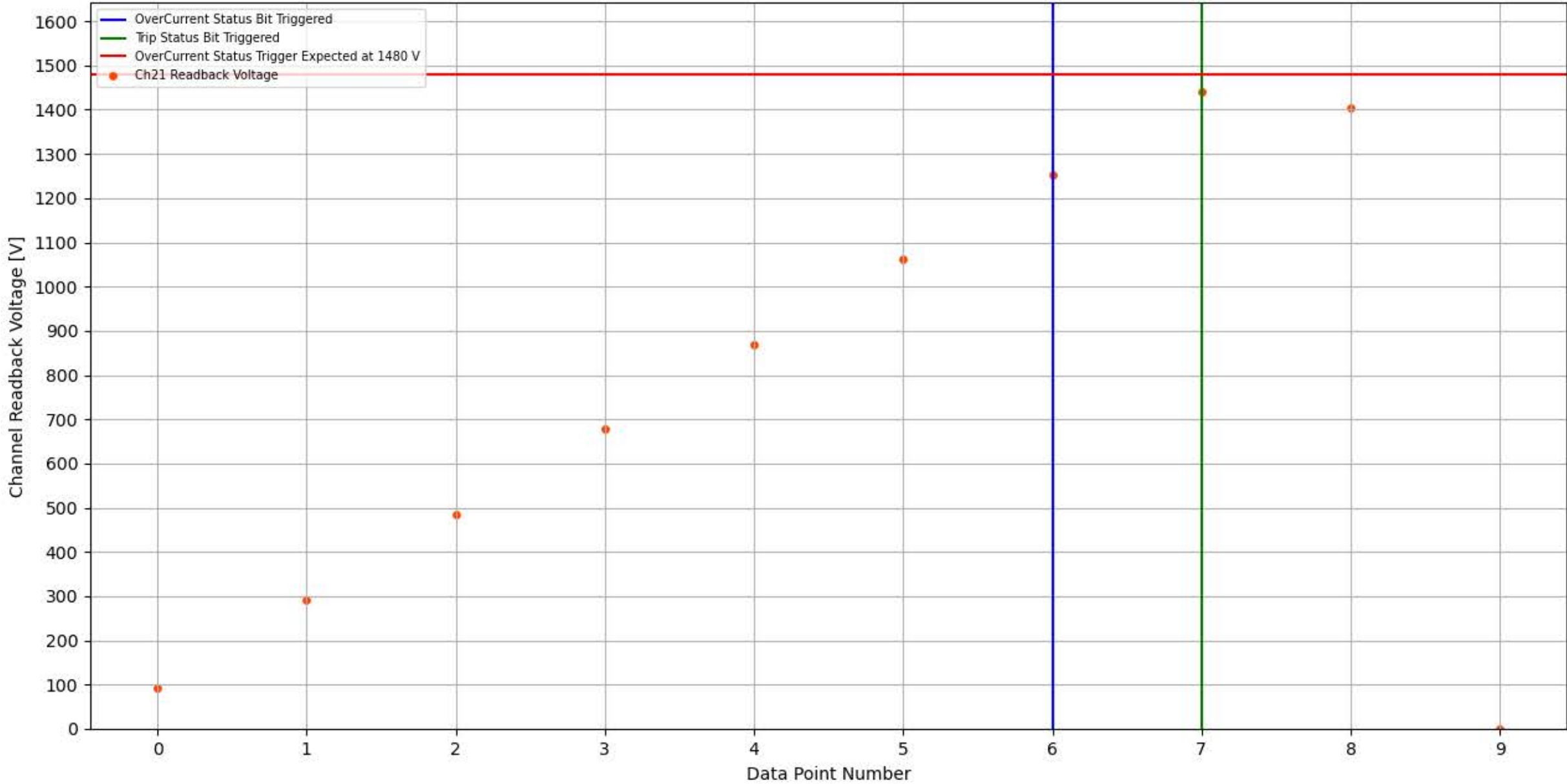
Module 352, Slot 2, Channel 21 Trip Test
