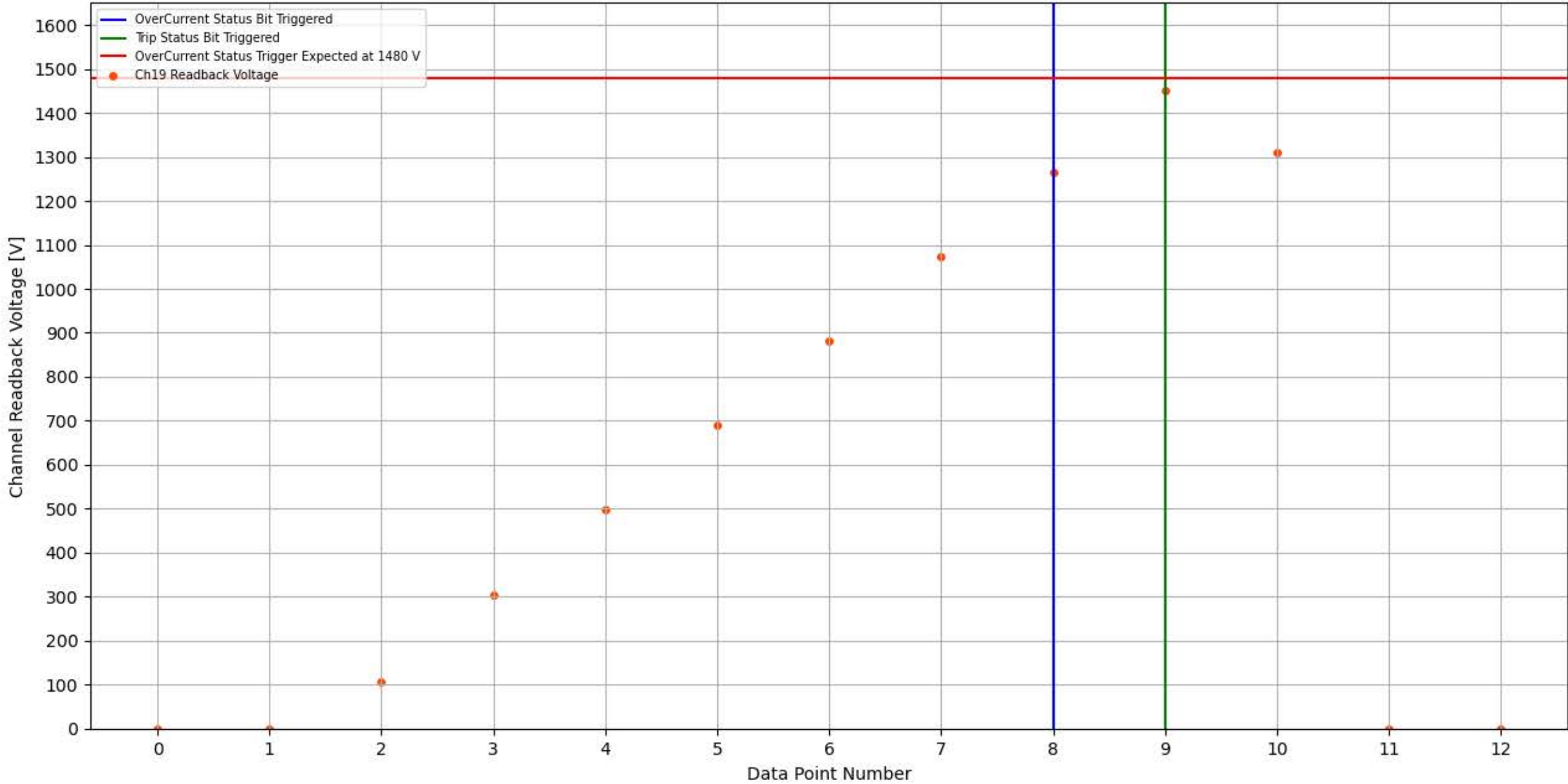
Module 352, Slot 2, Channel 19 Trip Test
