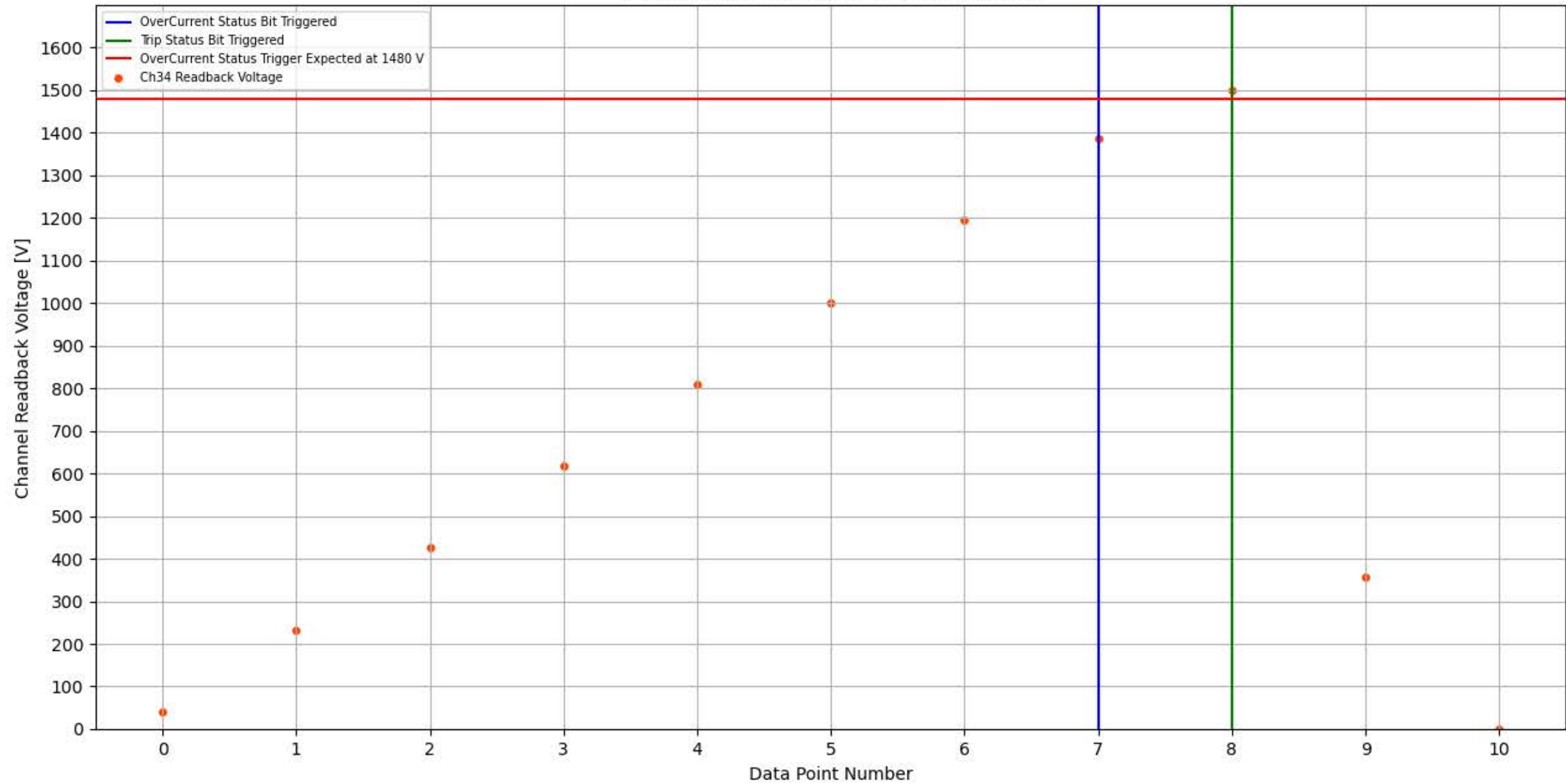
Module 352, Slot 2, Channel 34 Trip Test
