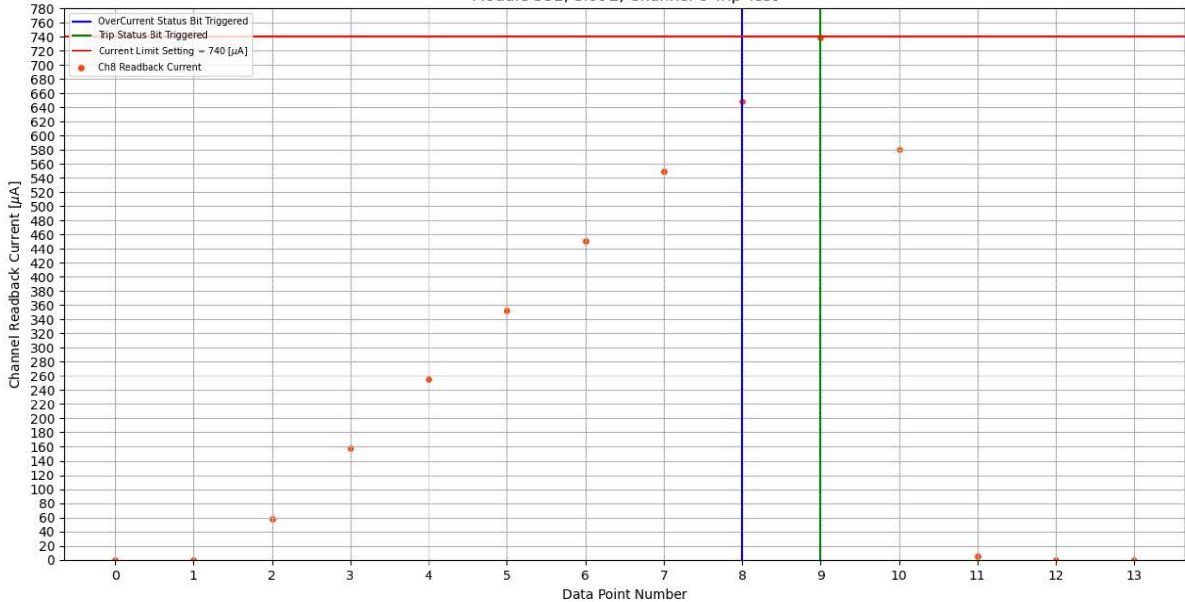
Module 352, Slot 2, Channel 8 Trip Test
