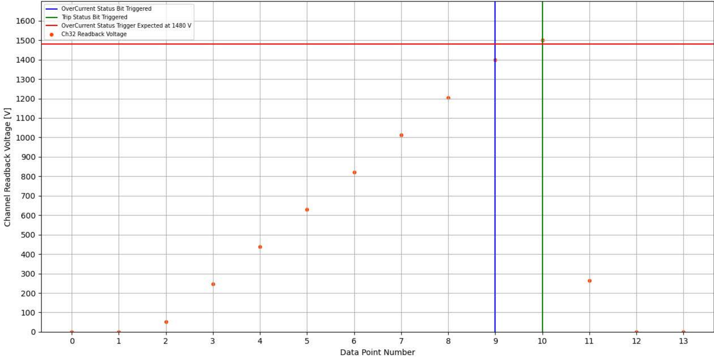
Module 352, Slot 2, Channel 32 Trip Test
