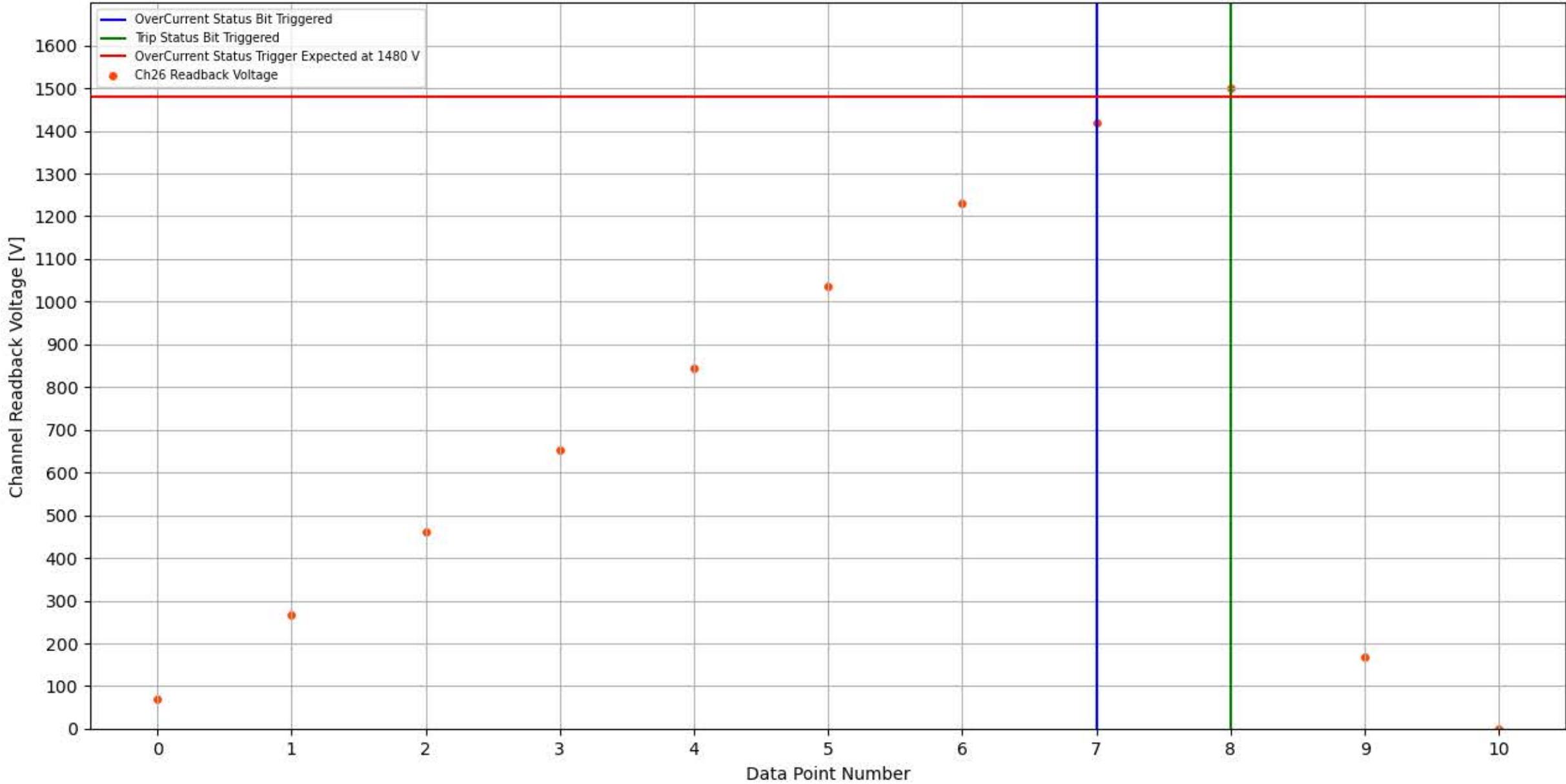
Module 352, Slot 2, Channel 26 Trip Test
