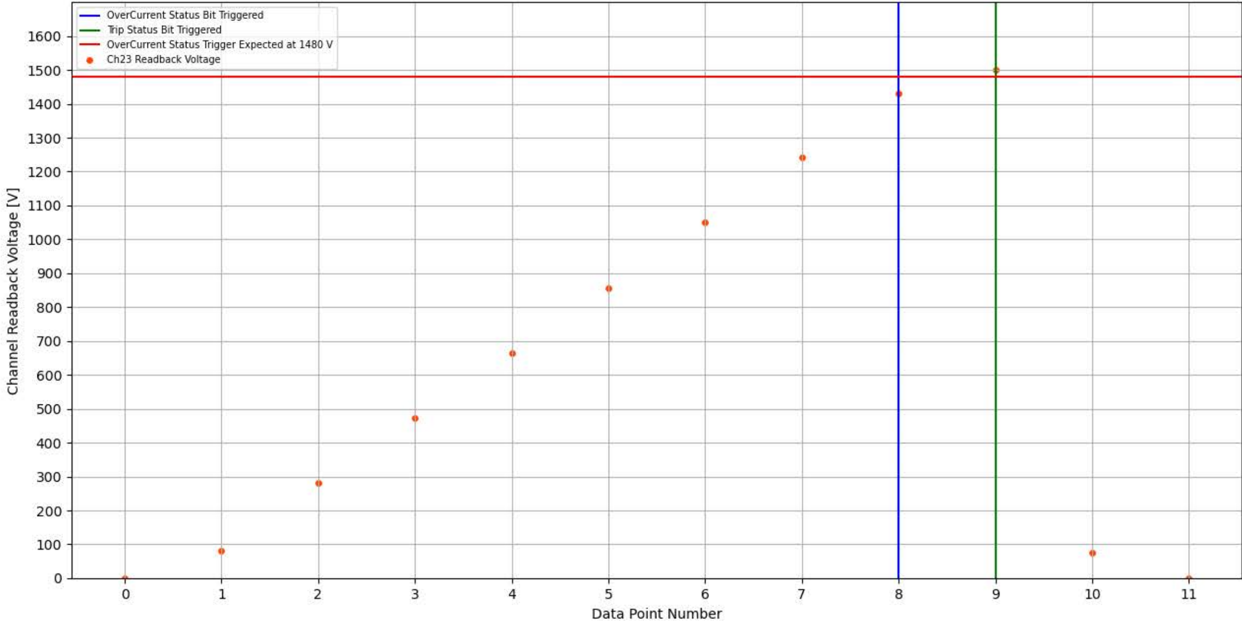
Module 352, Slot 2, Channel 23 Trip Test
