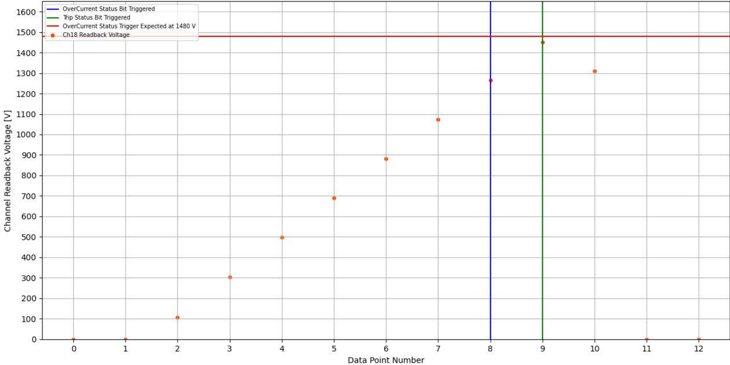
Module 352, Slot 2, Channel 18 Trip Test
