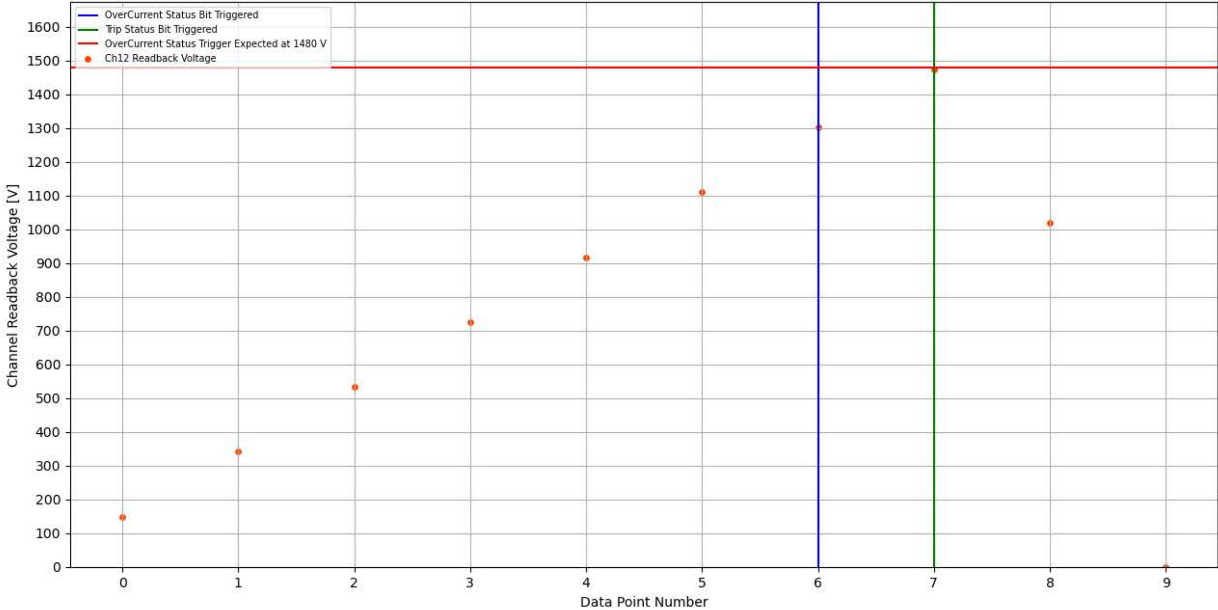
Module 352, Slot 2, Channel 12 Trip Test
