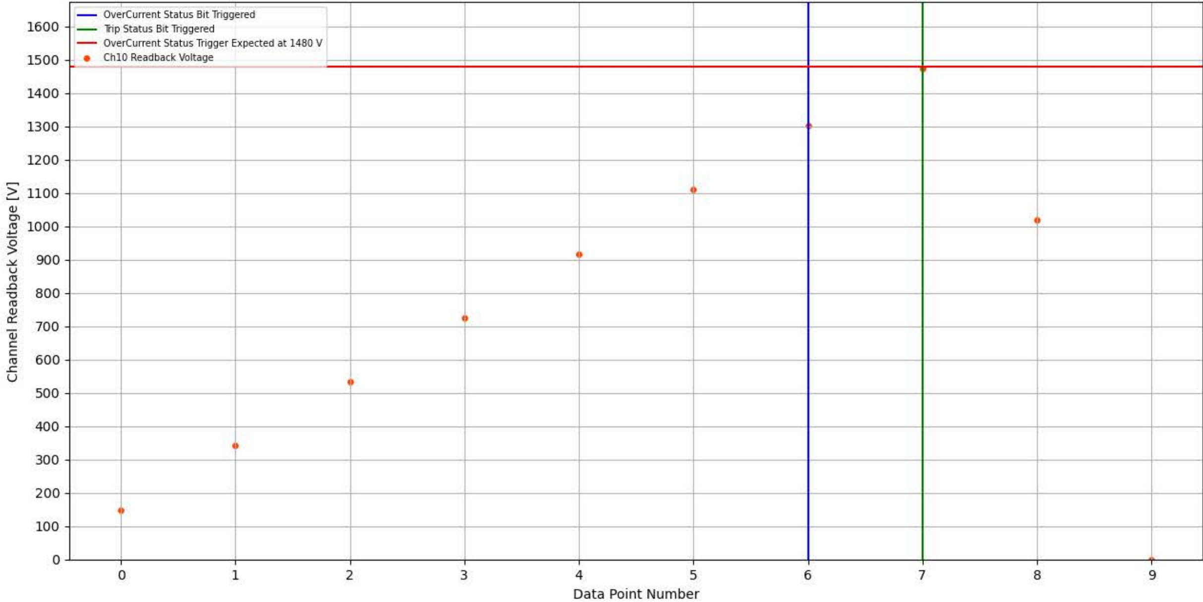
Module 352, Slot 2, Channel 10 Trip Test
