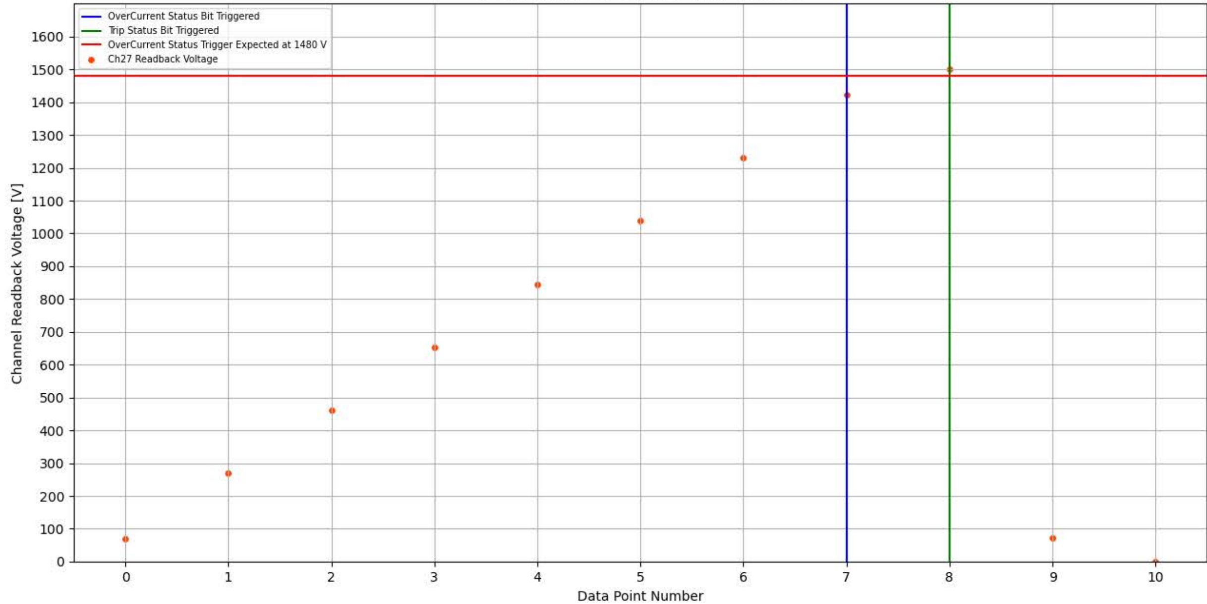
Module 352, Slot 2, Channel 27 Trip Test
