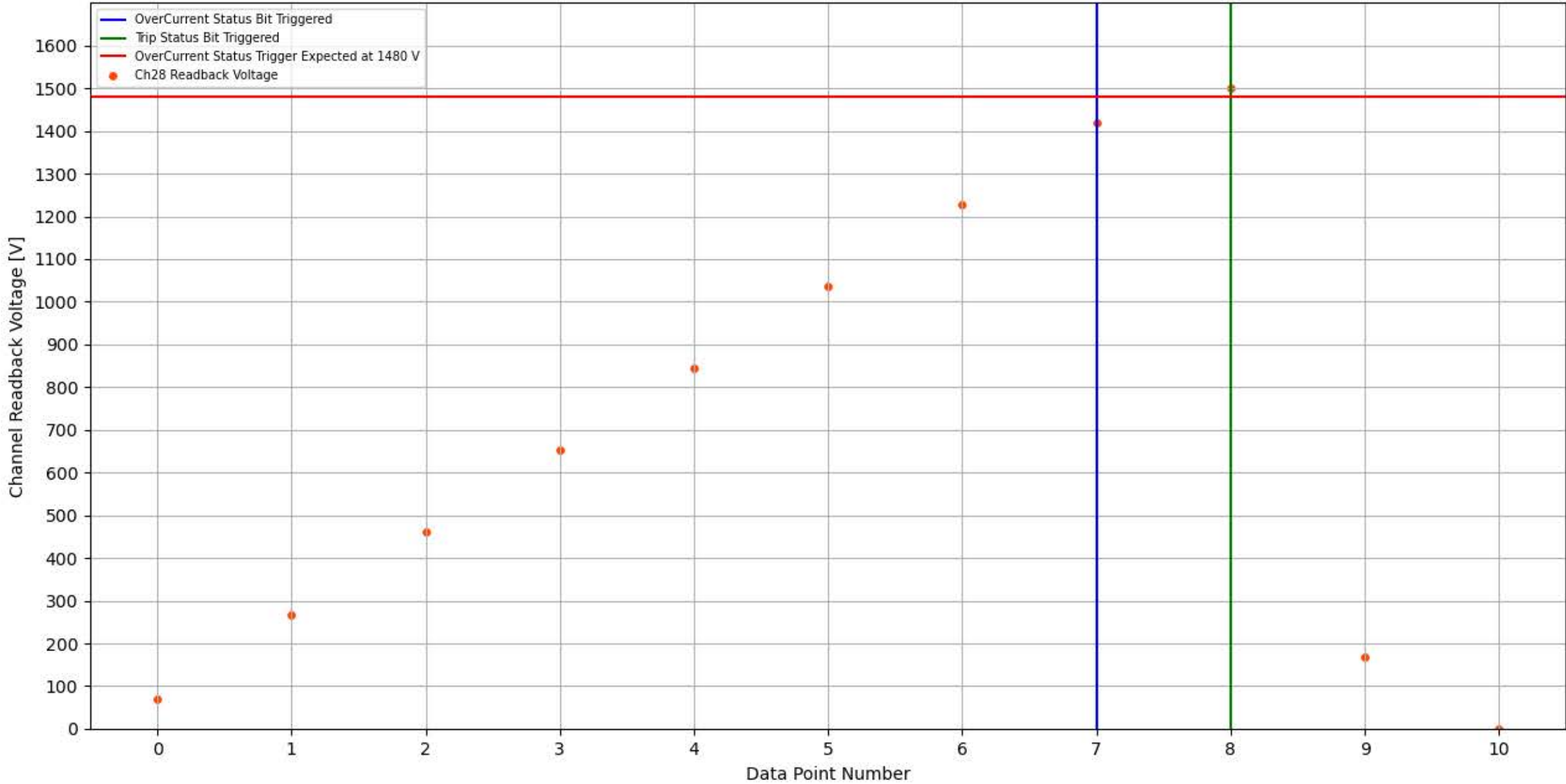
Module 352, Slot 2, Channel 28 Trip Test
