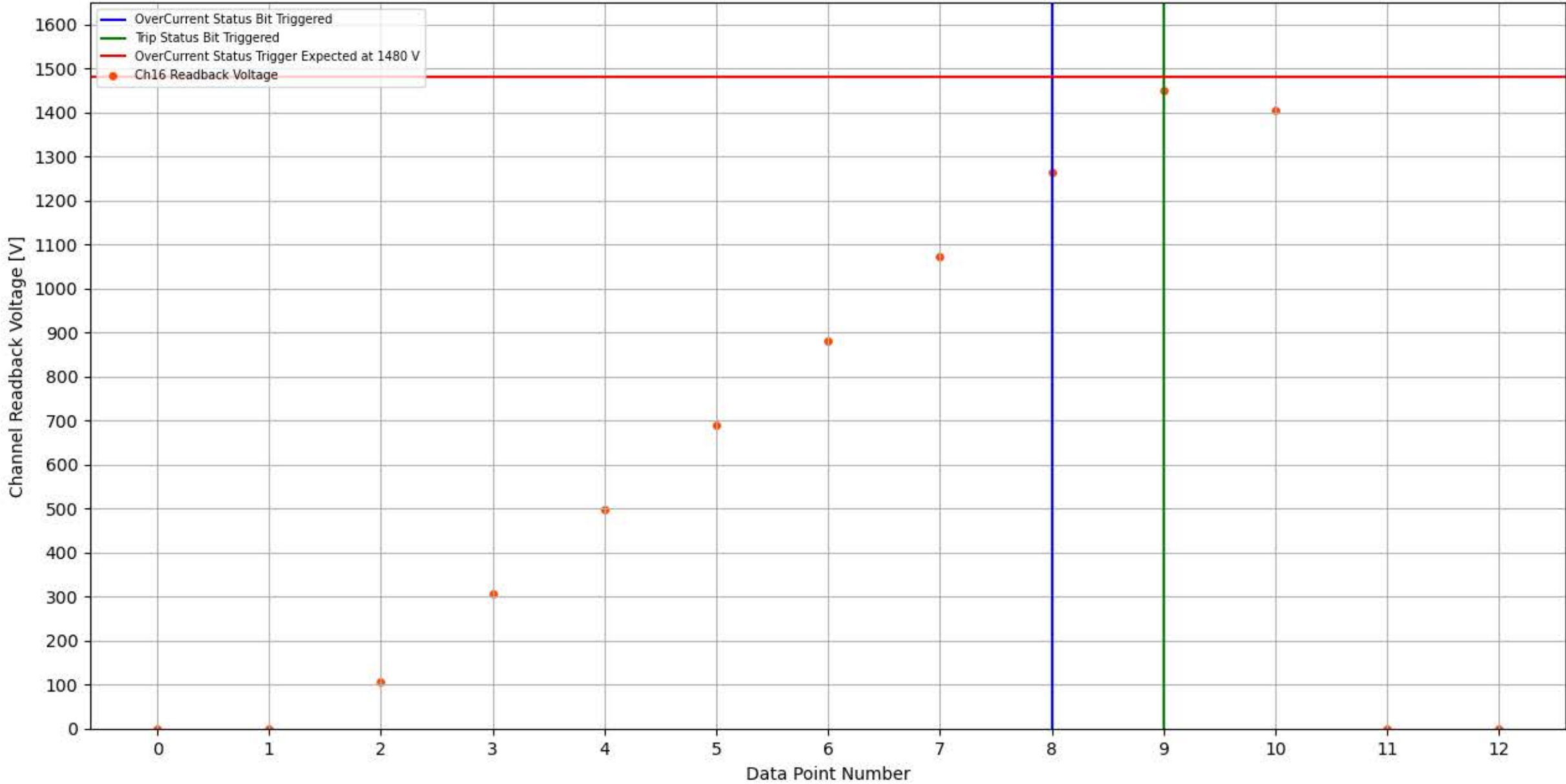
Module 352, Slot 2, Channel 16 Trip Test
