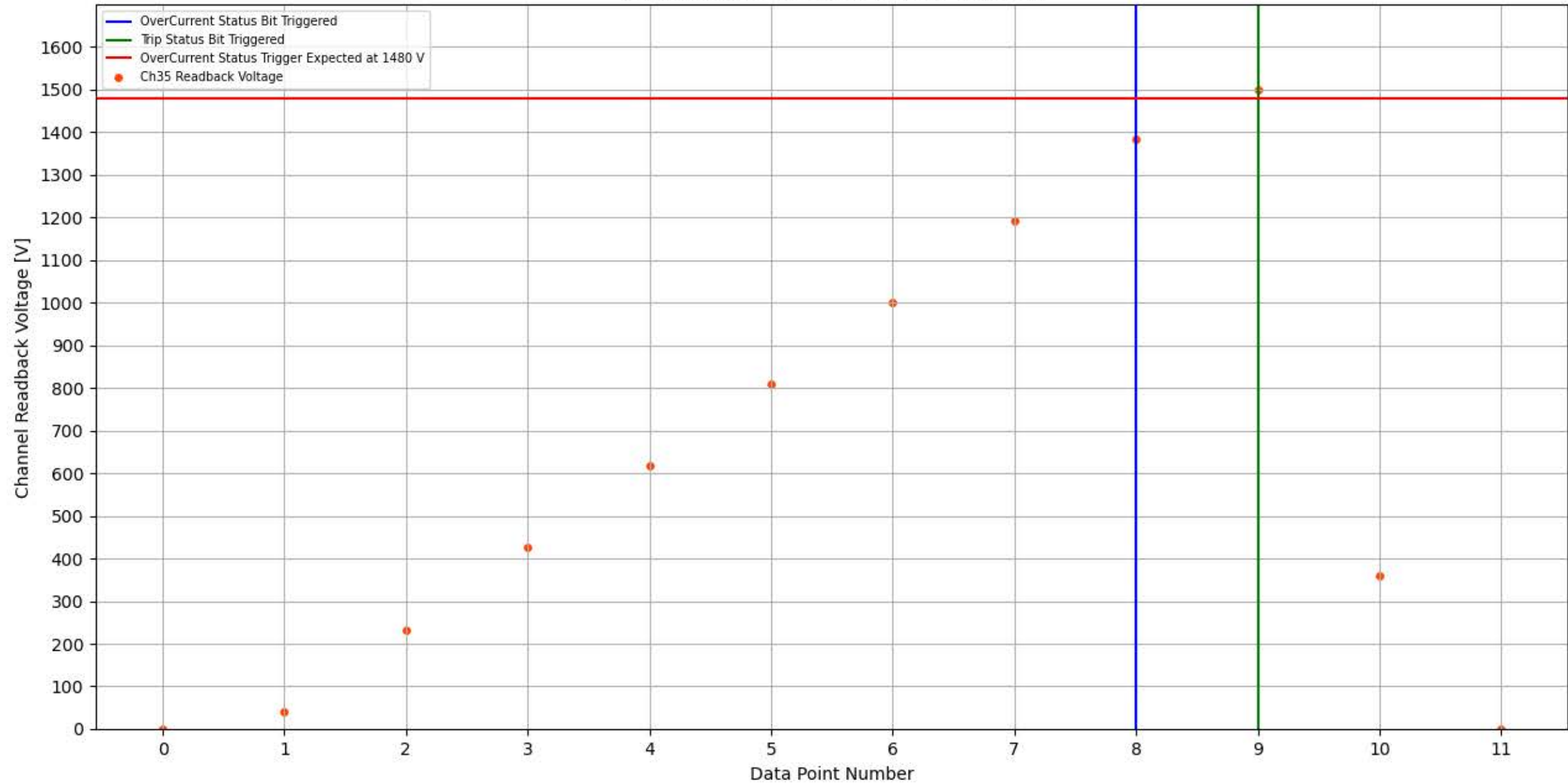
Module 352, Slot 2, Channel 35 Trip Test
