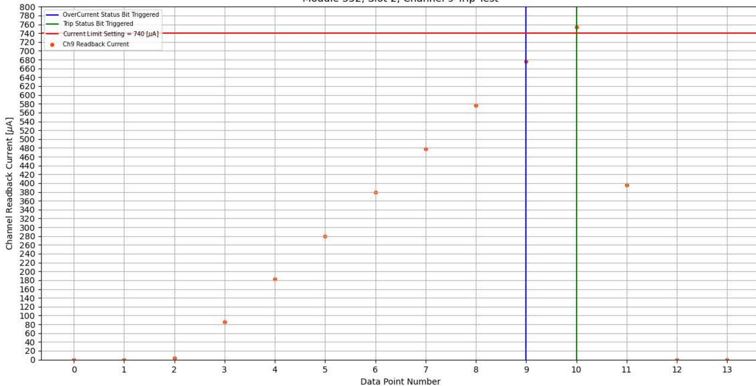
Module 352, Slot 2, Channel 9 Trip Test
